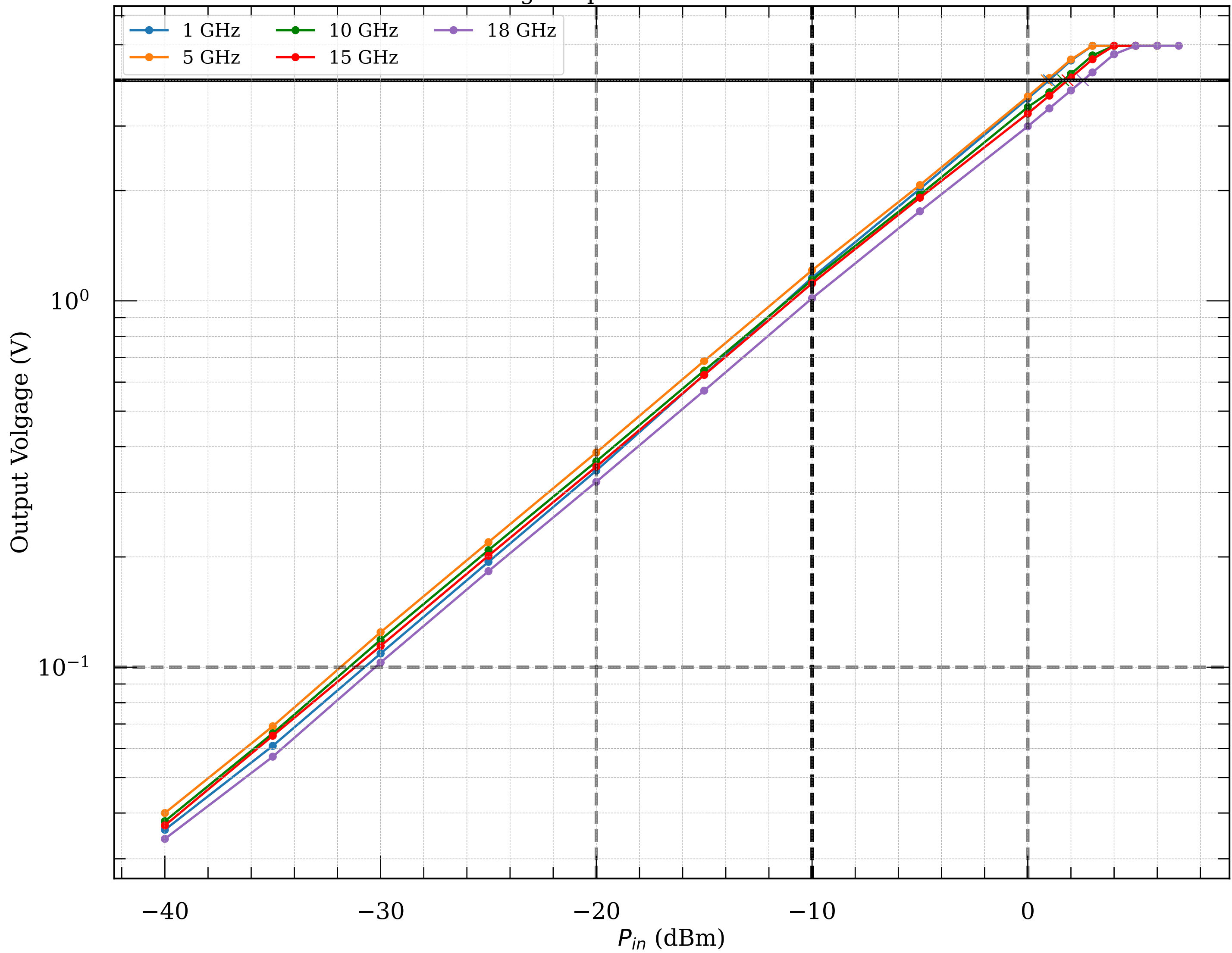
Measured voltage-to-power curve of detector module085
